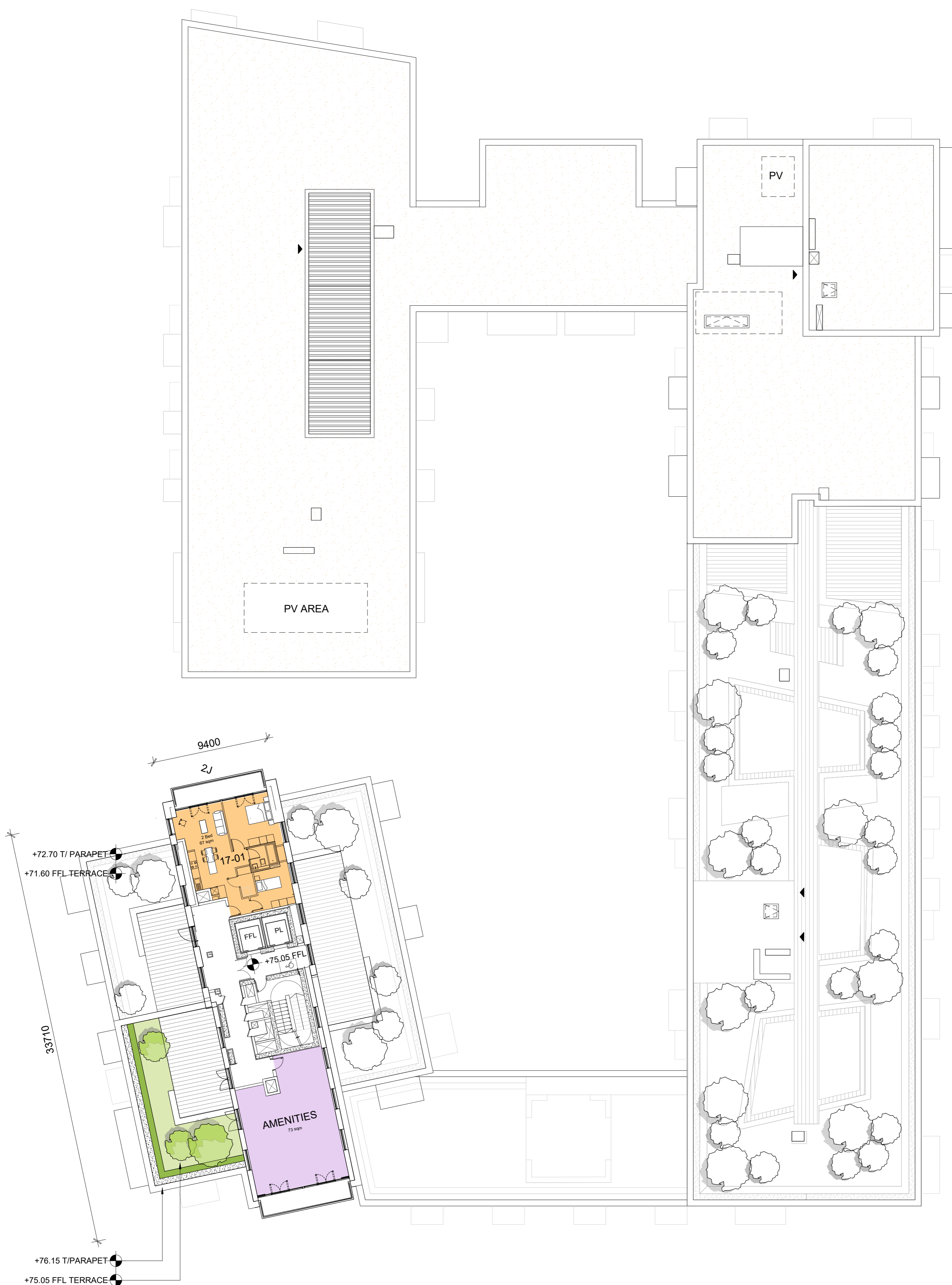
01 PW2 LEVEL 17 PLAN PL1217 SCALE 1:200
